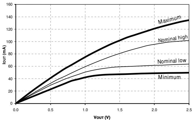
Figure 11: Pull-Down Characteristics
