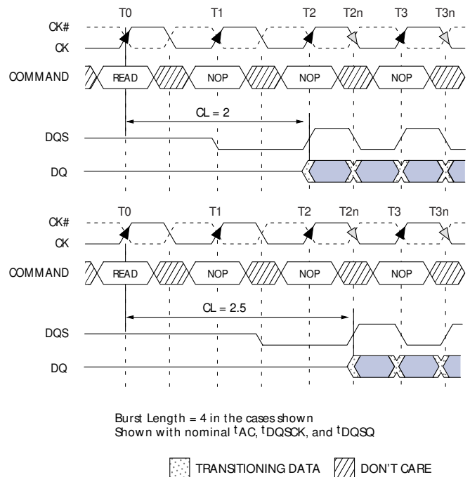
Figure 8: CAS Latency Diagram
