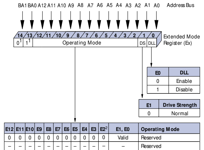
Figure 9: Extended Mode Register Definition Diagram
