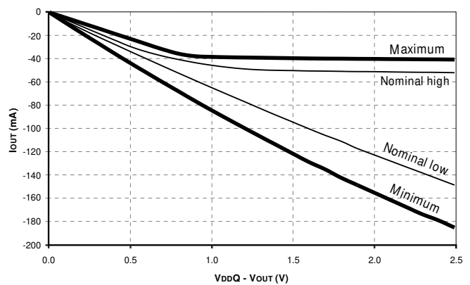
Figure 12: Pull-Up Characteristics
