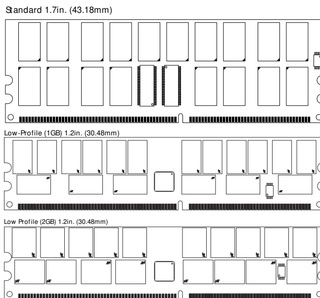
Figure 1: 184-Pin DIMM (MO-206)
