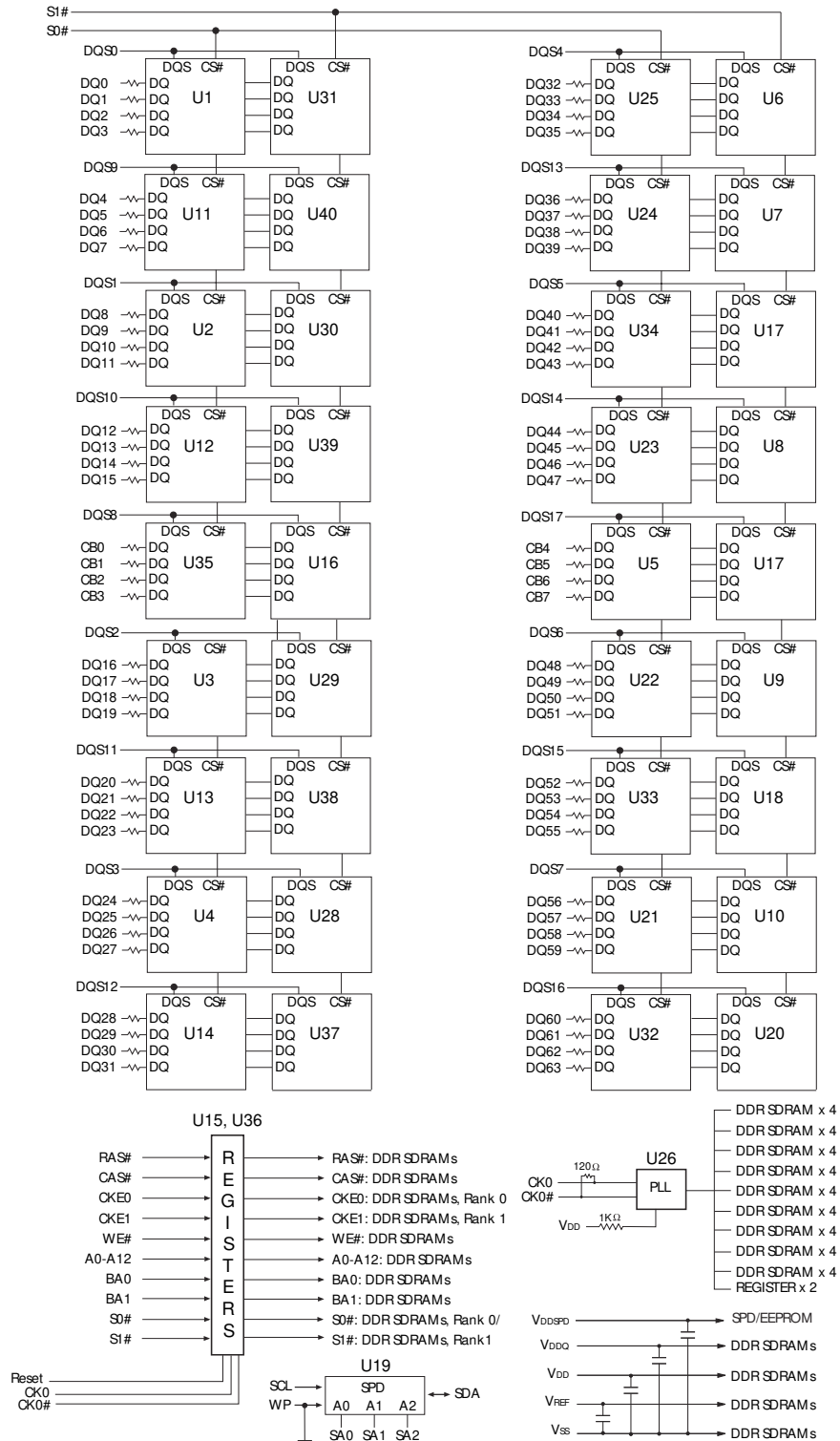
Figure 6: Low-Profile PCB Functional Block Diagram – 2GB
