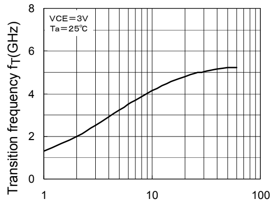
f_T-I_C
