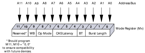
Figure 4: Mode Register Definition Diagram
