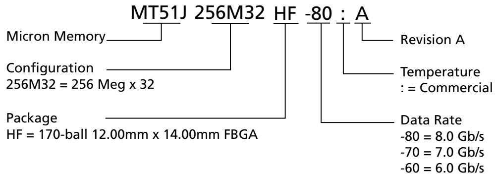
Figure 1: Part Numbering
