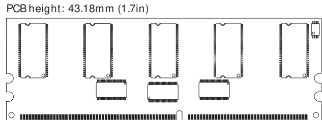
Figure 2: Standard-Height Layout (MO-206-CA R/C L)
