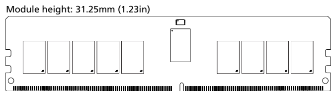
Figure 1: 288-Pin RDIMM (MO-309, R/C-E1, R/C-E2)
