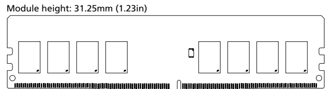
Figure 1: 288-Pin UDIMM (MO-309 R/C A1)
