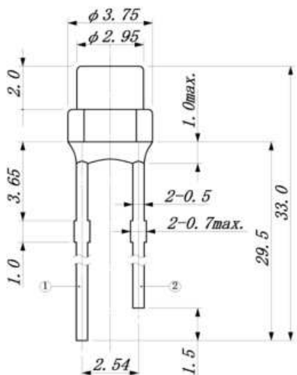
① Anode ② Cathode
