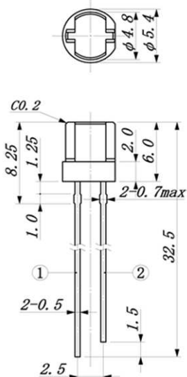
① Anode ② Cathode
