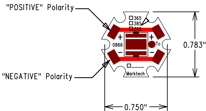
PCB - Star Board MTSM365UV4-F30115S
