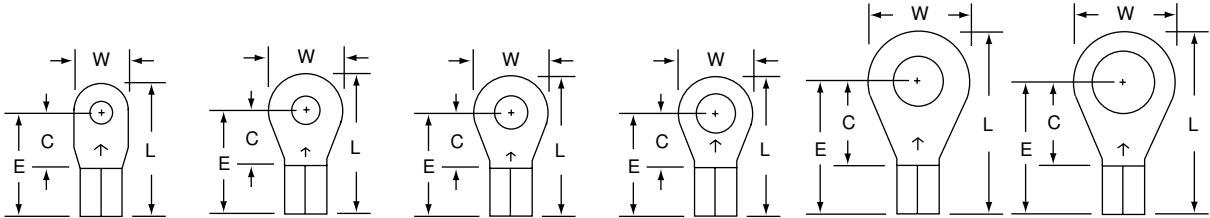
MU10-4R/S MU10-6R MU10-8R MU10-10R MU10-14R/S MU10-516R/S Stud Size 4 6 8 10 1/4 5/16 Wire Range 12-10 12-10 12-10 12-10 12-10 12-10
