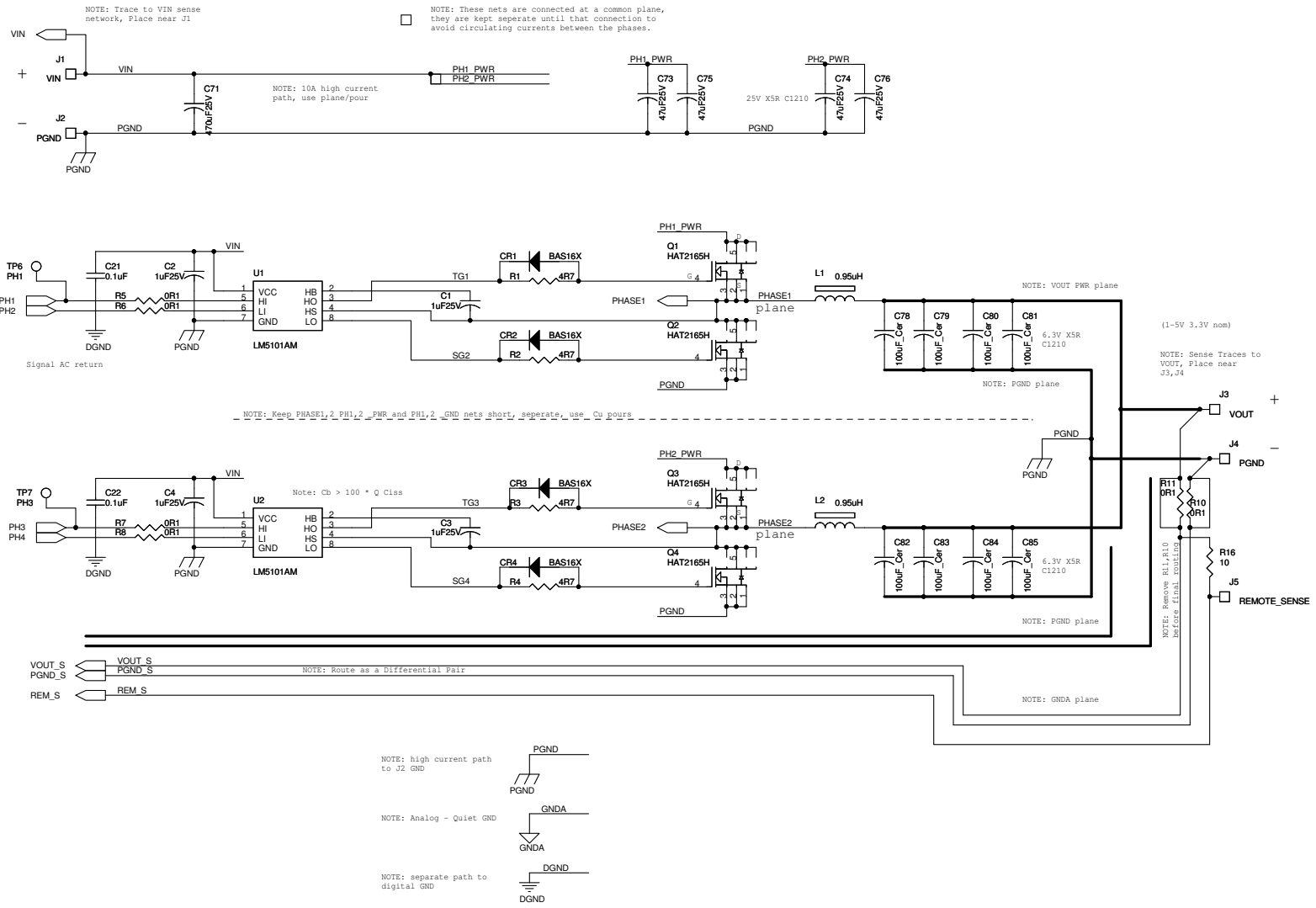
Figure 17. Si8250 Multi-Phase POL Target Board Schematic (Power)
