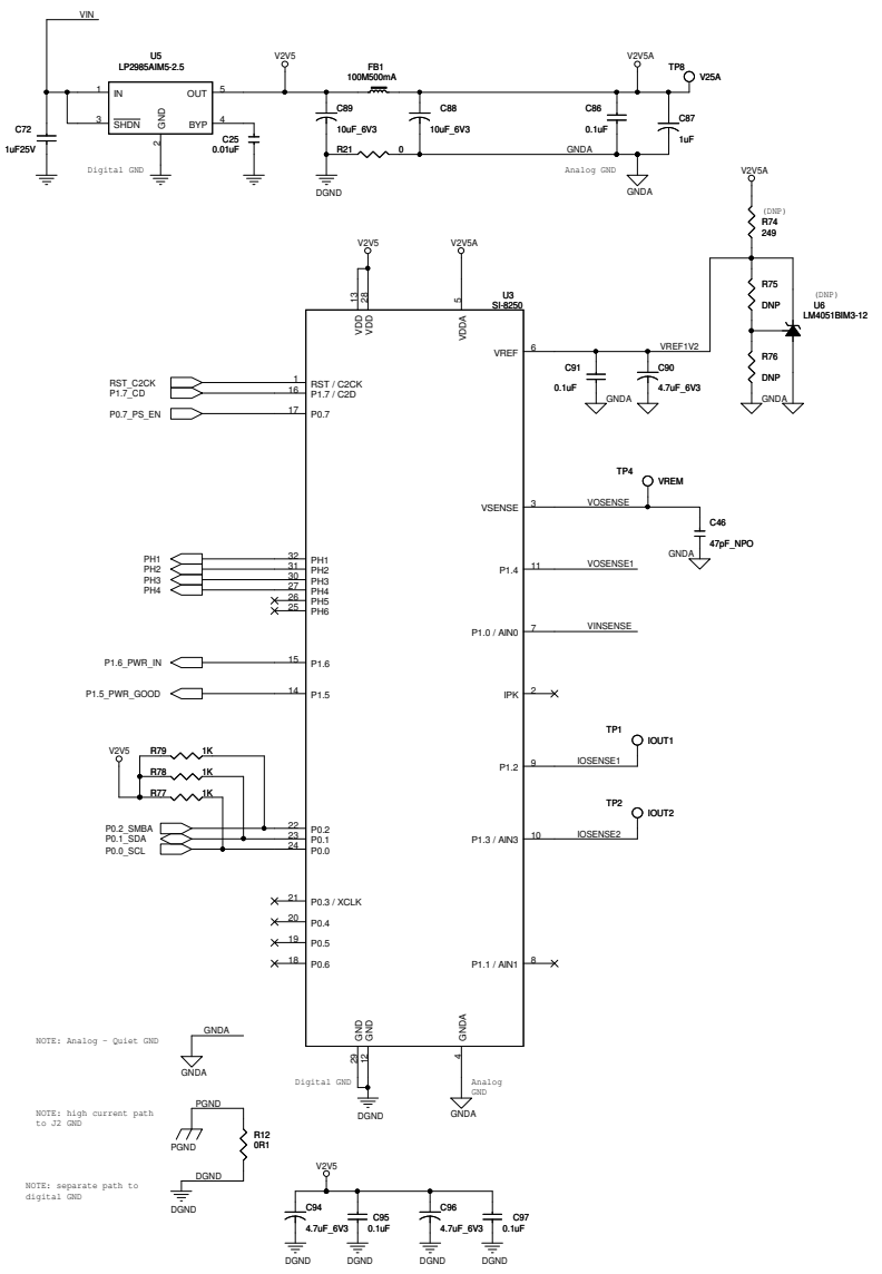
Figure 18. Si8250 Multi-Phase POL Target Board Schematic (Control)
