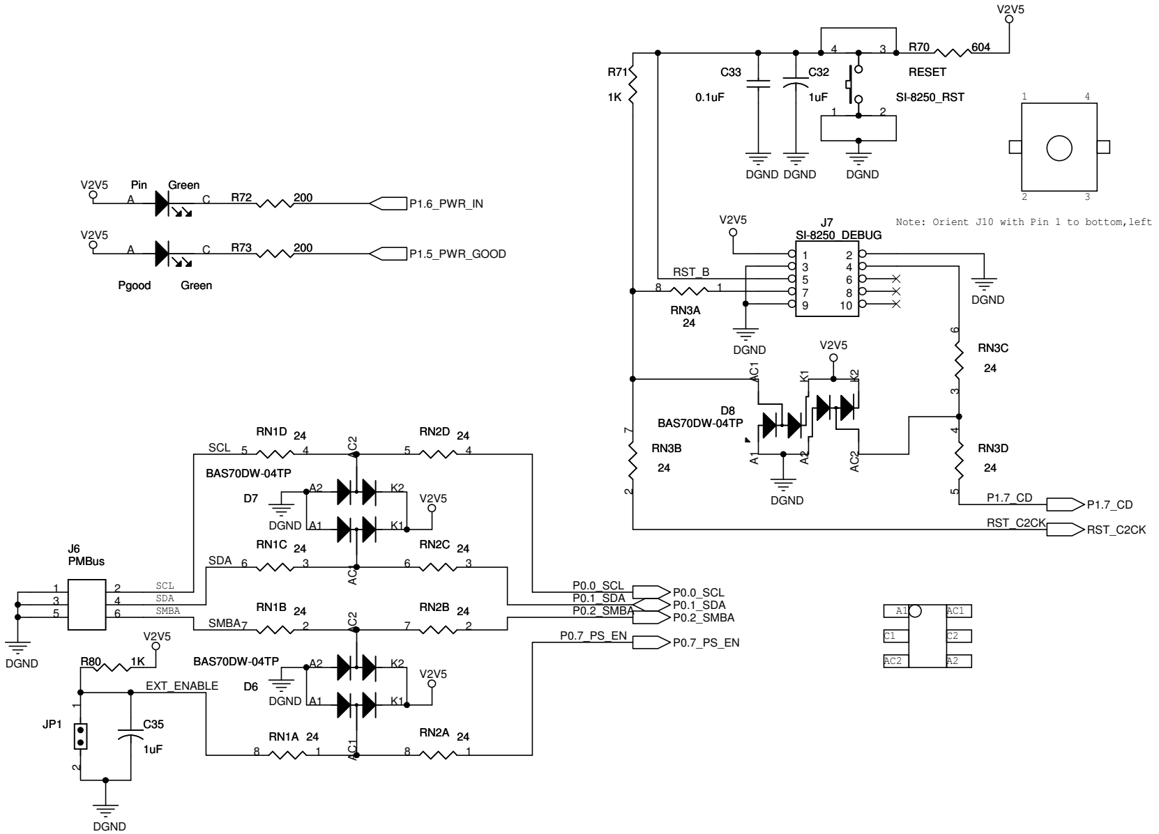
Figure 19. Si8250 Multi-Phase POL Target Board Schematic (Debug)
