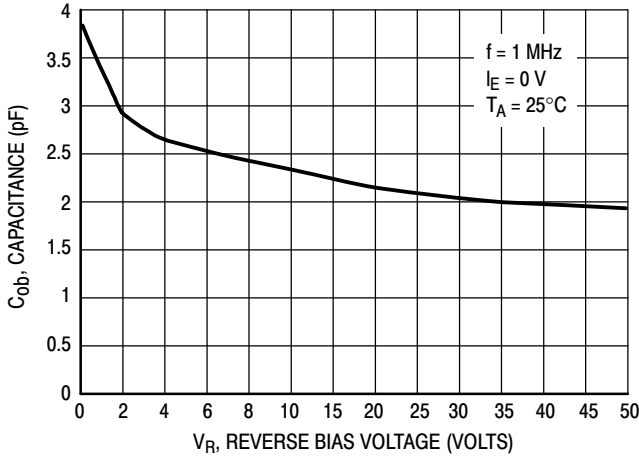
Figure 19. Output Capacitance
