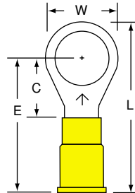
MV10-38R/S 3/8 12-10
