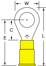
MV10-516R/S 5/16 12-10
