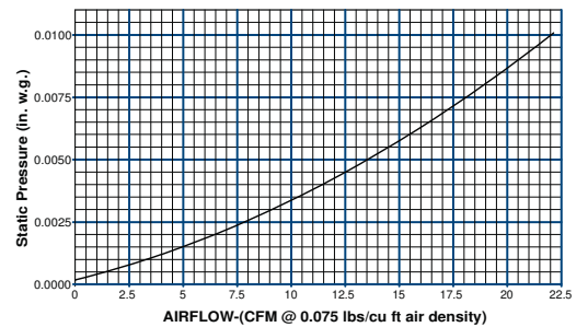
P-Q CURVE, DUCTED FLOW
