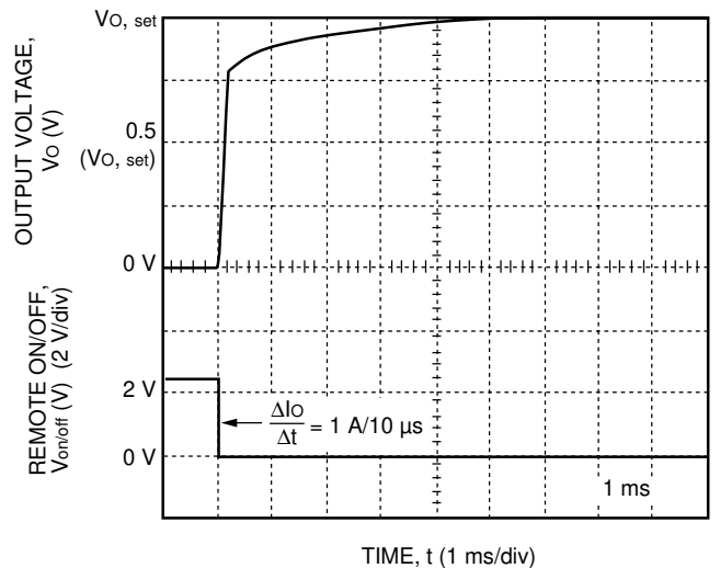
Figure 16. MW010A Typical Output Voltage Start-Up Waveform with Remote On/Off; I_o = 0.8 (I_{o,max}) ; V_I = 48\text{ V} ; T_A = 25\text{ }^\circ\text{C}
