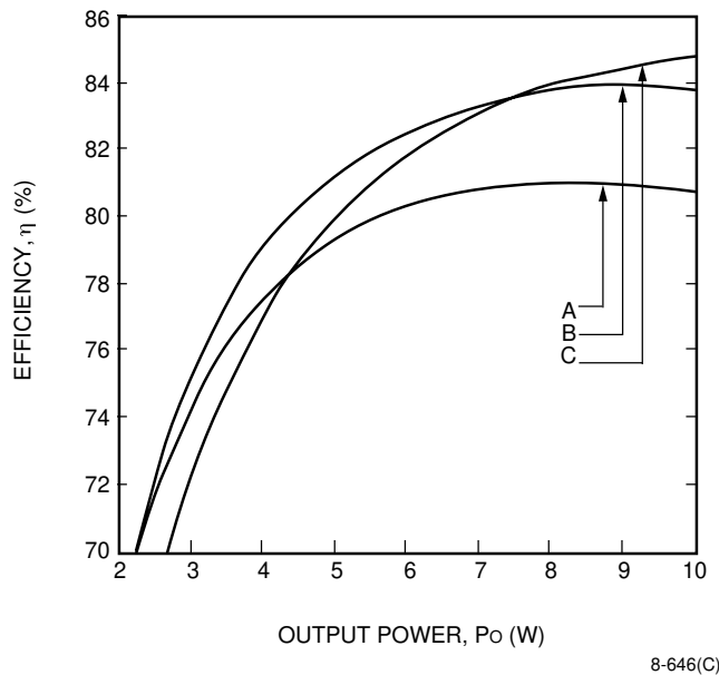
Figure 8. MW010A, B, C Typical Converter Efficiency as a Function of Output Power; V_I = 48\text{ V} ; T_A = 25\text{ }^\circ\text{C}
