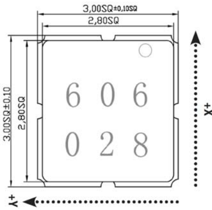
Figure 2 Top View
