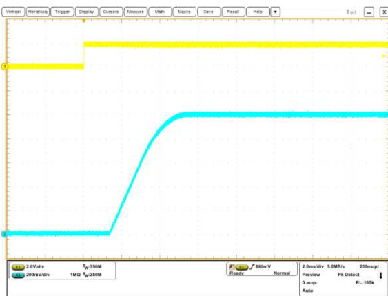
On/Off Enable Delay (Vin=5.0V, Vout=1.0V, Iout=6A, Cload=400uF) Trace1=Enable, Trace2=Vout, 2 ms/div
