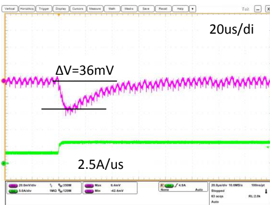
Step Load Transient Response (Vin=5.0V, Vout=0.7V, Cload=400uF, Iout=3A to 6A) Trace 3=Vout, 20 mV/div, Trace 4=Iout, 5A/div.
