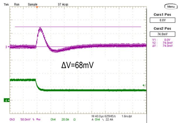
Step Load Transient Response (Vin=12.0V, Vout=1.8V, Load=760uF, Iout=30 to 15A, 1.0A/us) Trace 3=Vout, 50mV/div, Trace 4=Iout, 20A/div.
