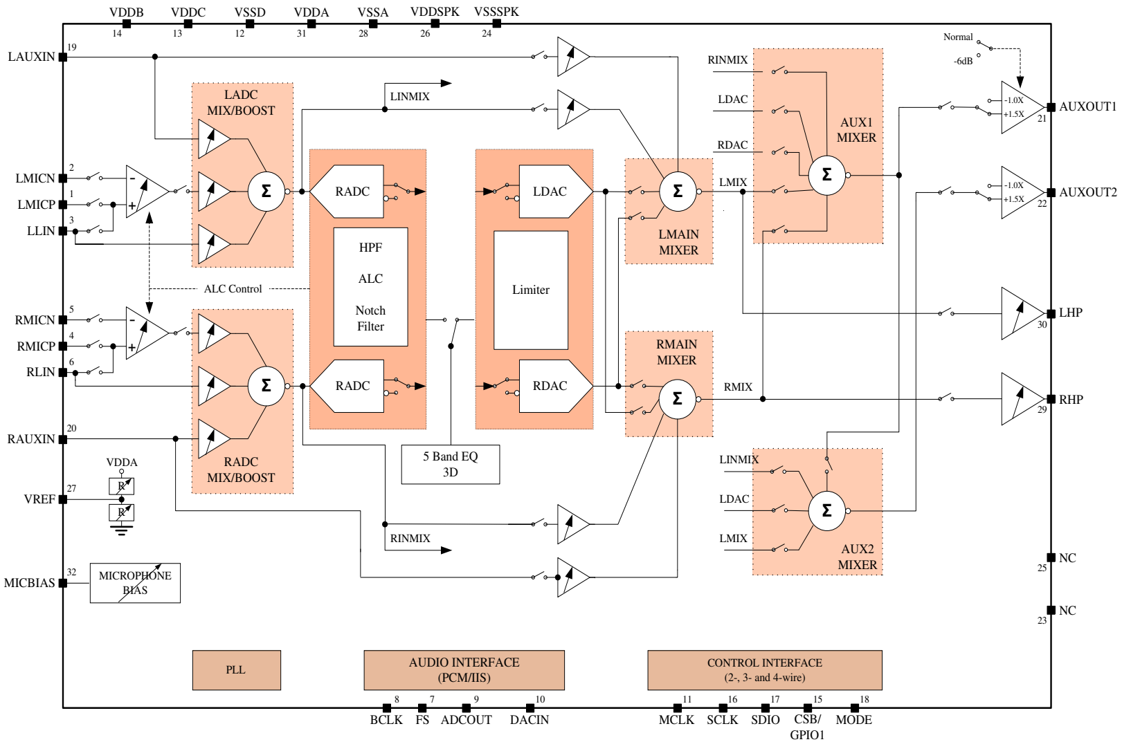
Figure 1: NAU8820 Block Diagram
