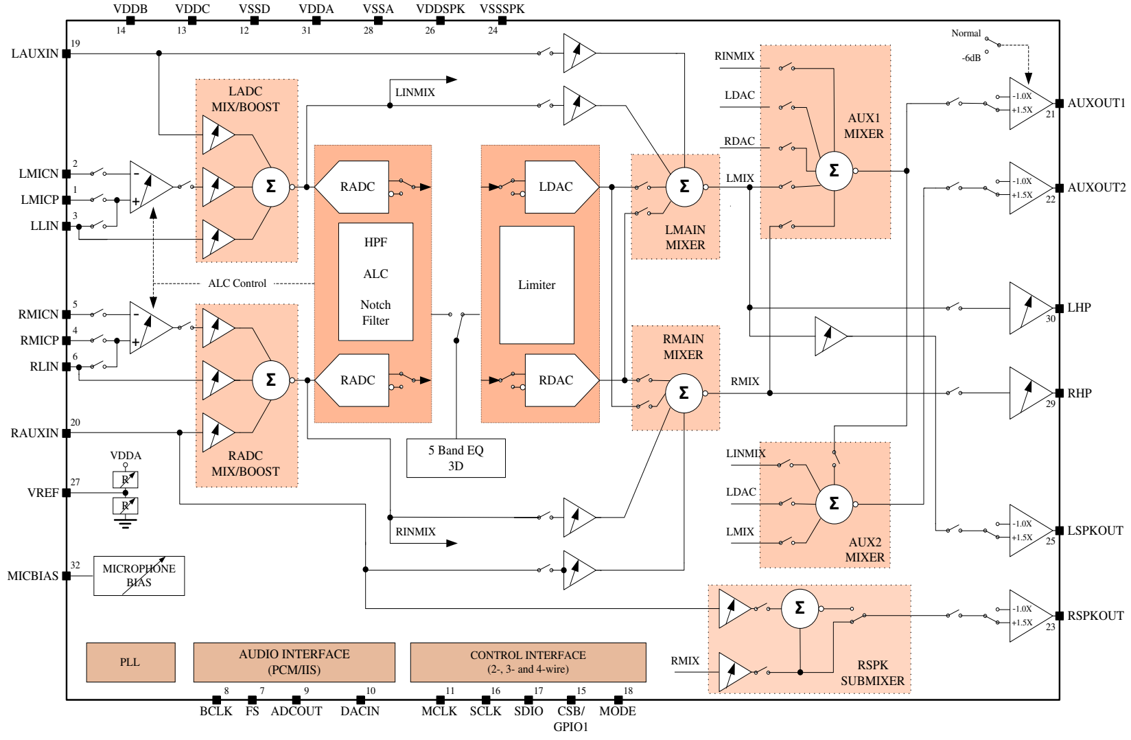
Figure 1: NAU8822 Block Diagram
