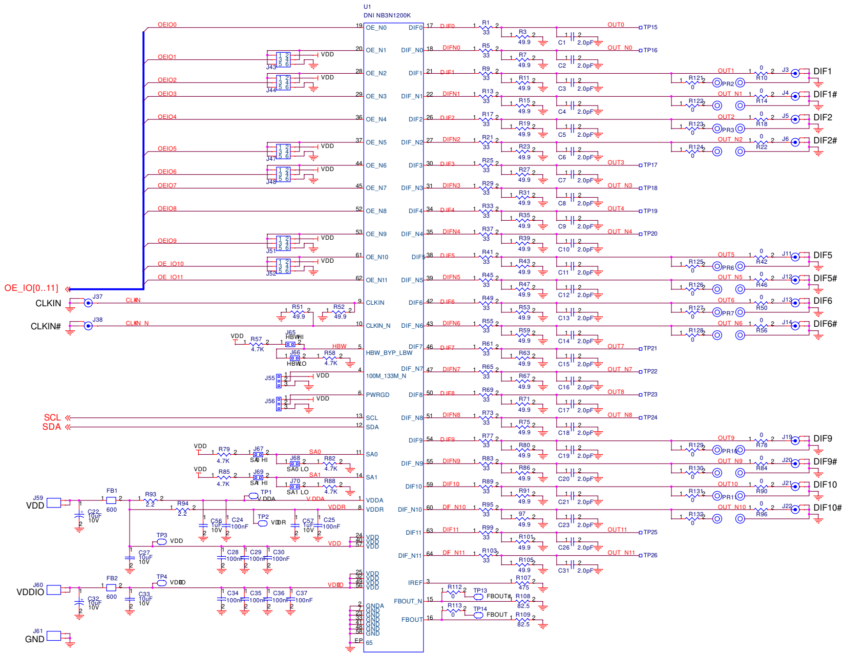
Figure 12. NB3N1200KMNGEVB & NB3W1200LMNGEVB Board Schematic
