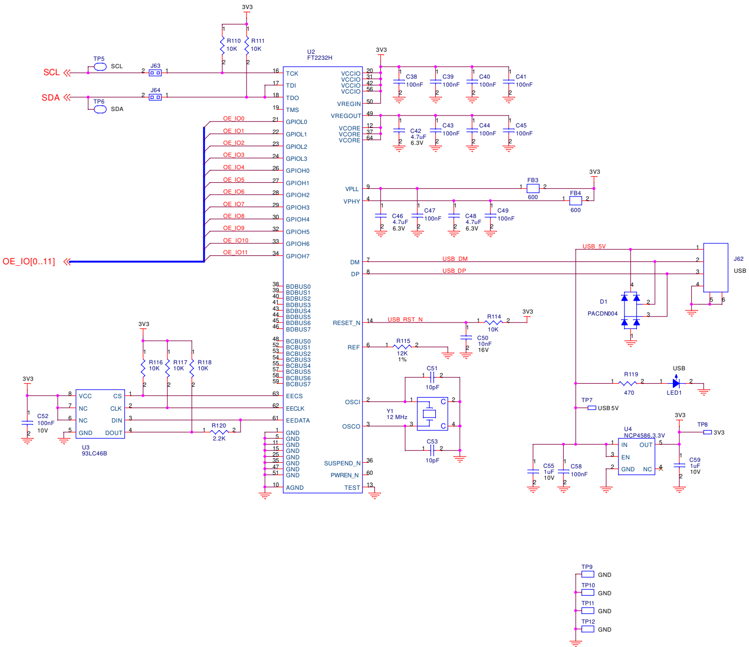
Figure 13. USB Circuitry Schematic
