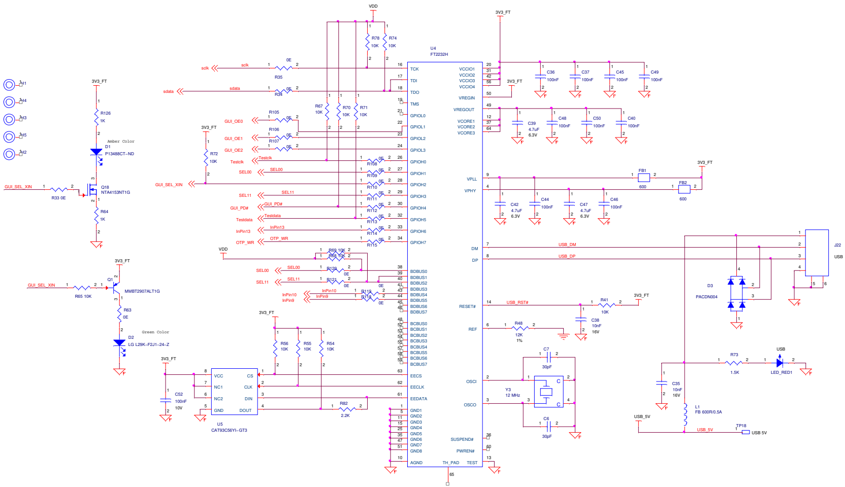
Figure 10. Main Board Schematic (2 of 3)
