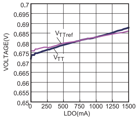
V_{TT} LDO Sink Current Load Regulation
