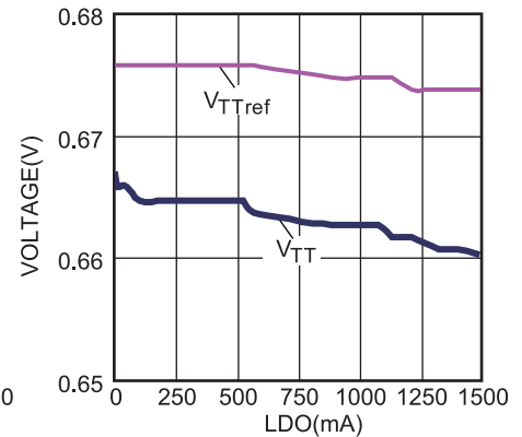
V_{TT} LDO Source Current Load Regulation
