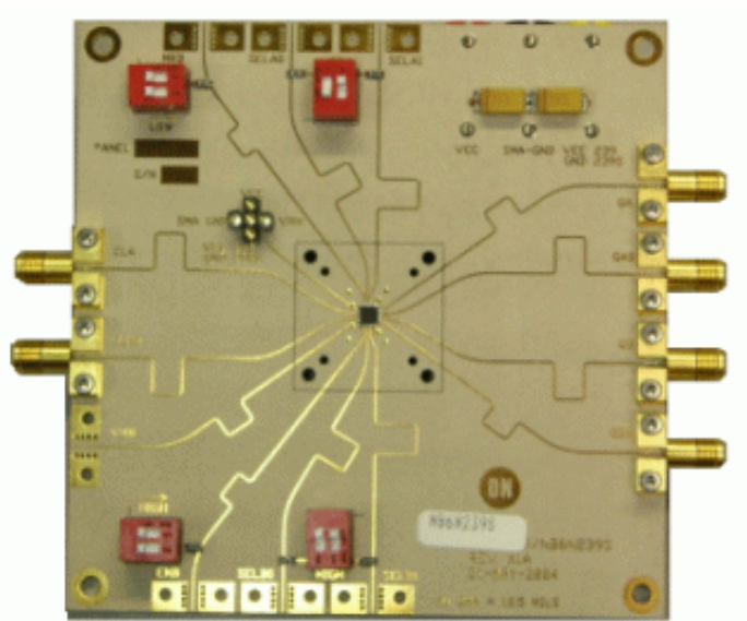
Figure 1. Evaluation Board
