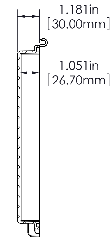
SECTION C-C SCALE 1 : 3
