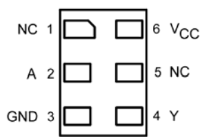
Figure 4. MicroPak™ (Top Through View)
