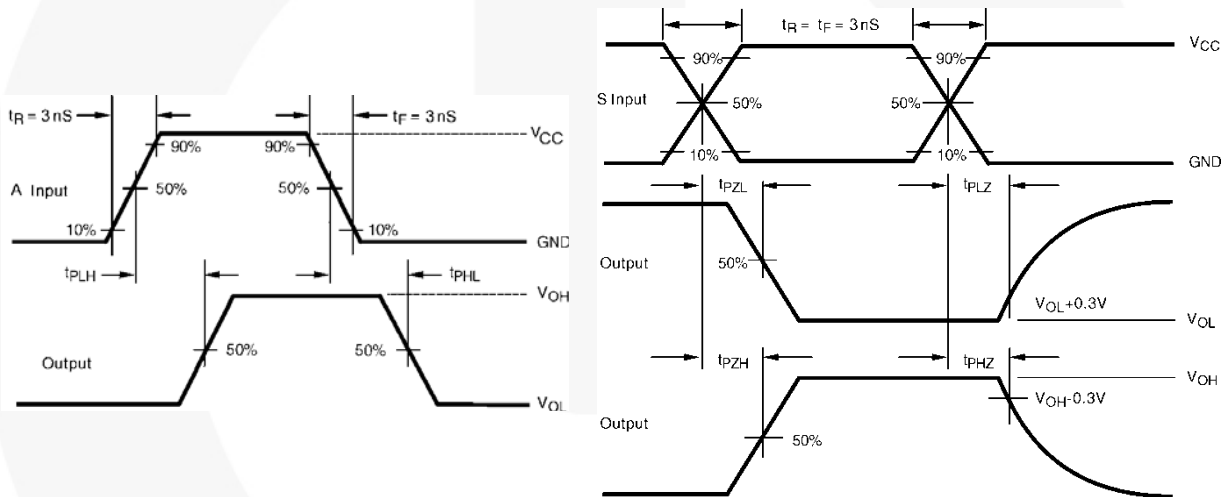
Figure 6. AC Waveforms
