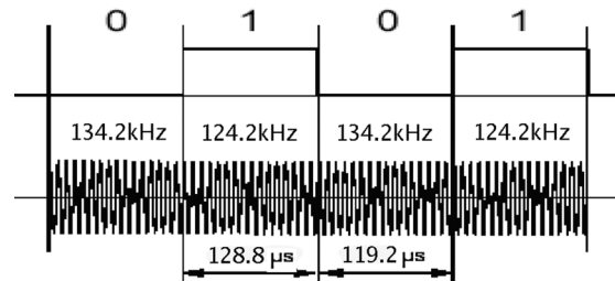
Figure 2: FSK Transmission Used During the Read Phase
