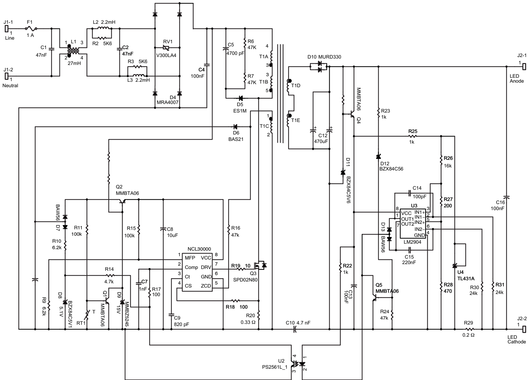
Figure 30. Wide Input Main, 4-15 LED 350 mA Load Schematic
