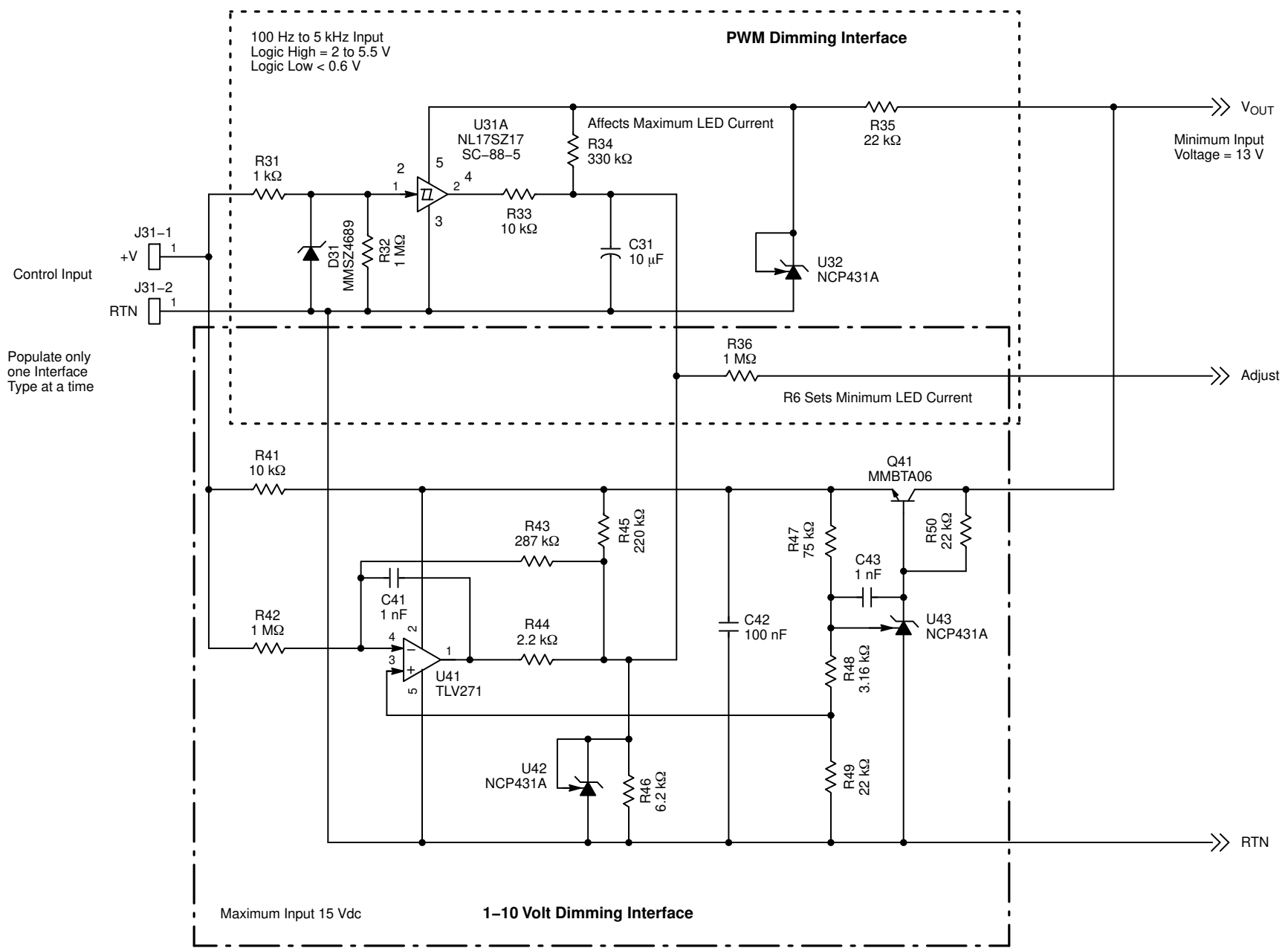
Figure 4. Dimming Control Schematic
