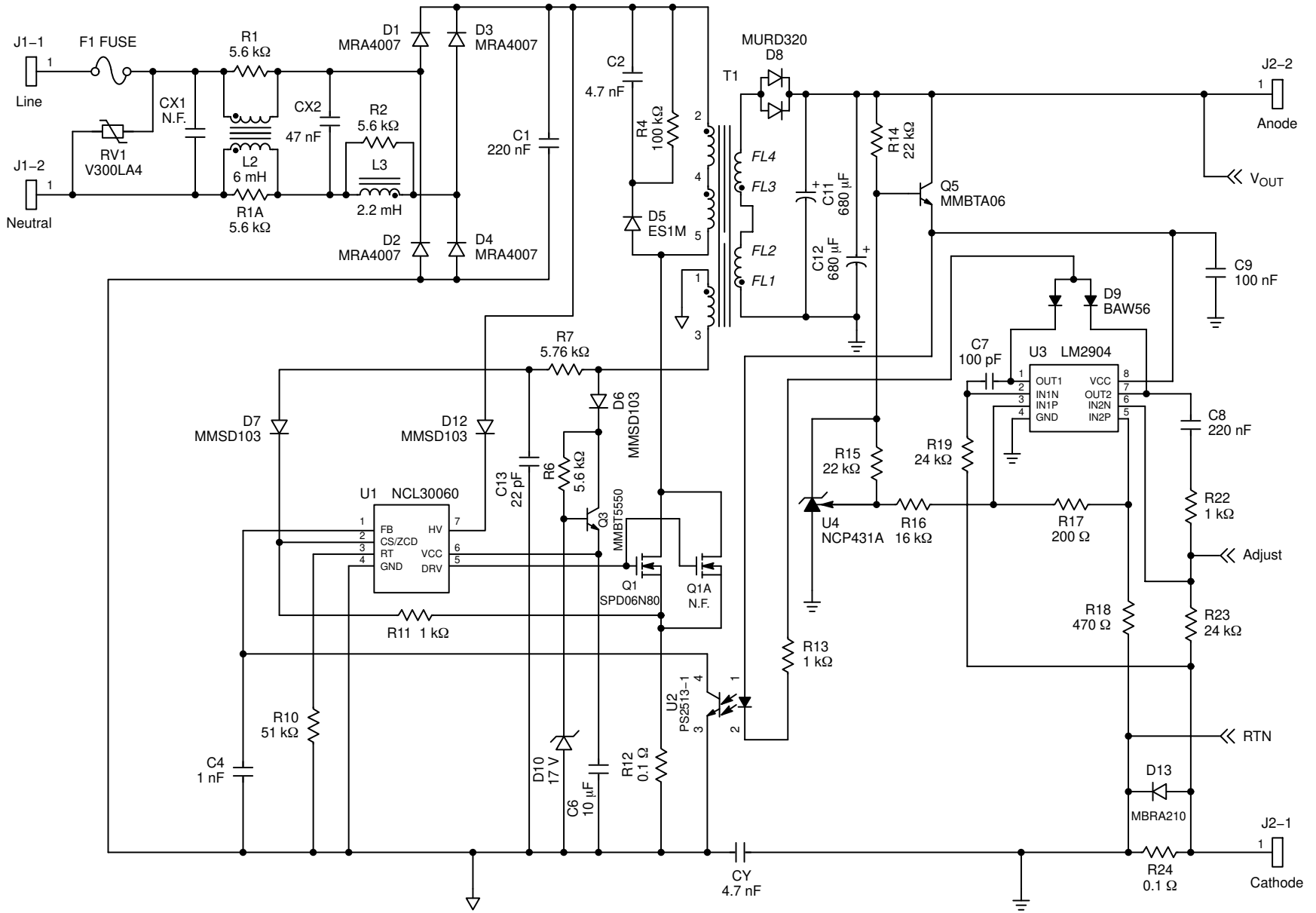
Figure 3. Power Stage Schematic
