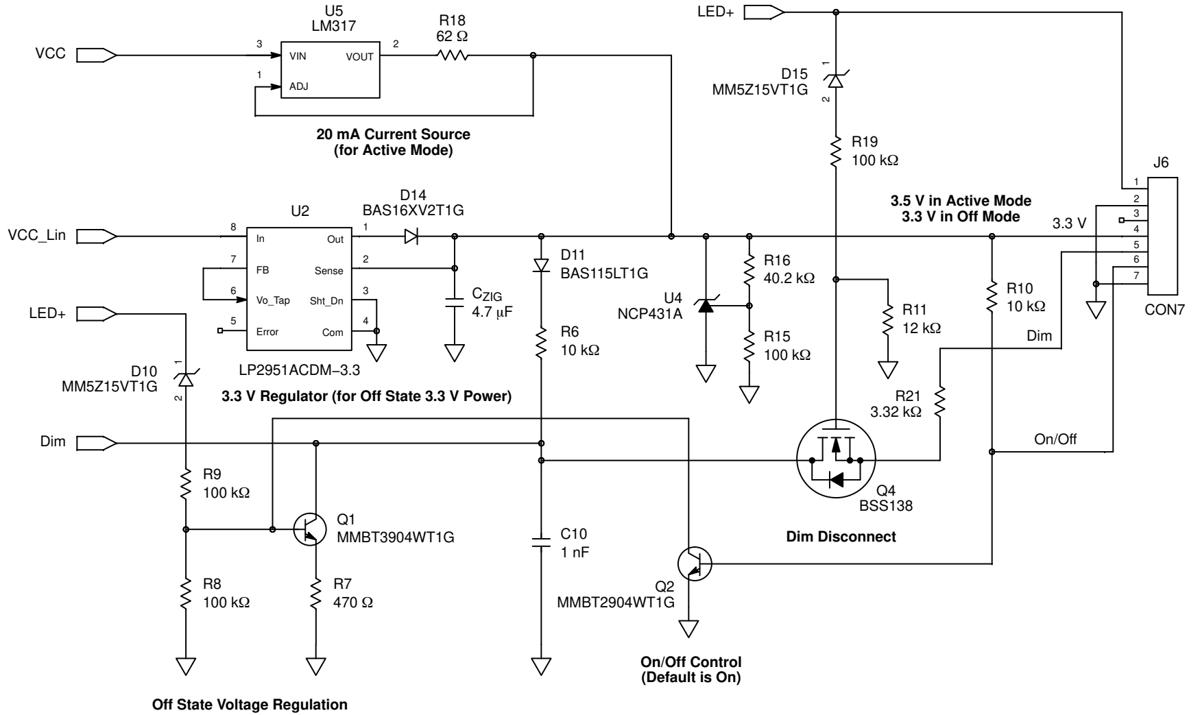
Figure 5. Interface Schematic
