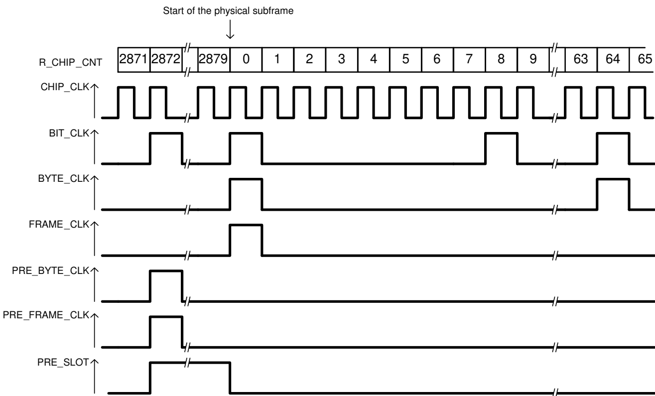
Figure 19. Timing Signals
