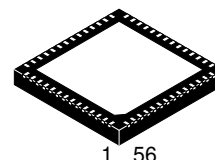
QFN56 8x8, 0.5P CASE 485CN
