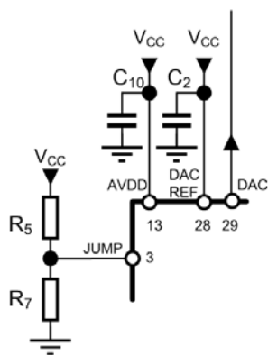
Figure 11. DAC Interface
