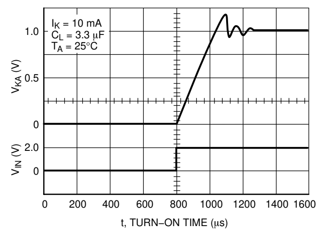
Figure 20. Turn-On Time
