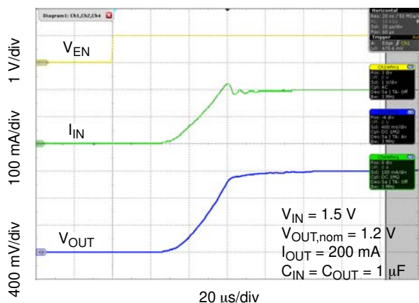
Figure 27. Enable Turn-on Response, C_{OUT} = 1 \mu\text{F} , I_{OUT} = 200 \text{ mA}
