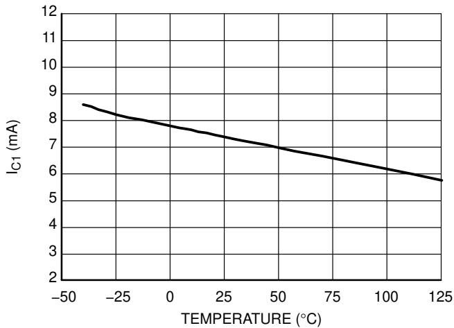
Figure 7. Internal Startup Current Source, V_{CC} = 10\text{ V} versus Temperature
