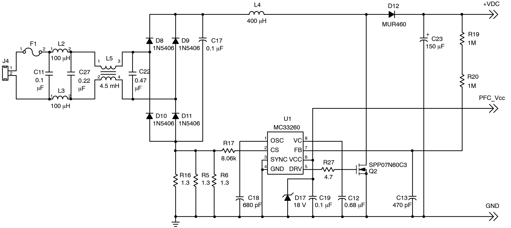
Figure 10. NCP1230 Demo Board Schematic – PFC section
