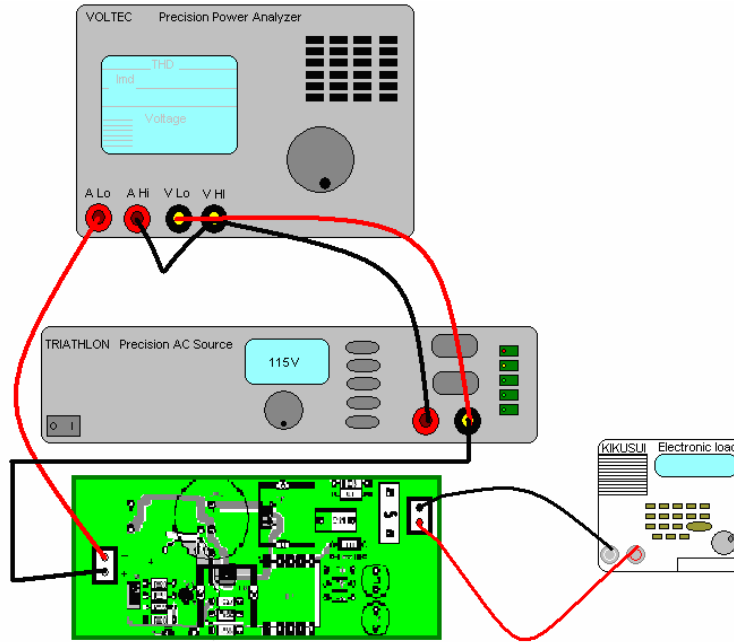
Figure 9. NCP1230GEVB Test Setup
