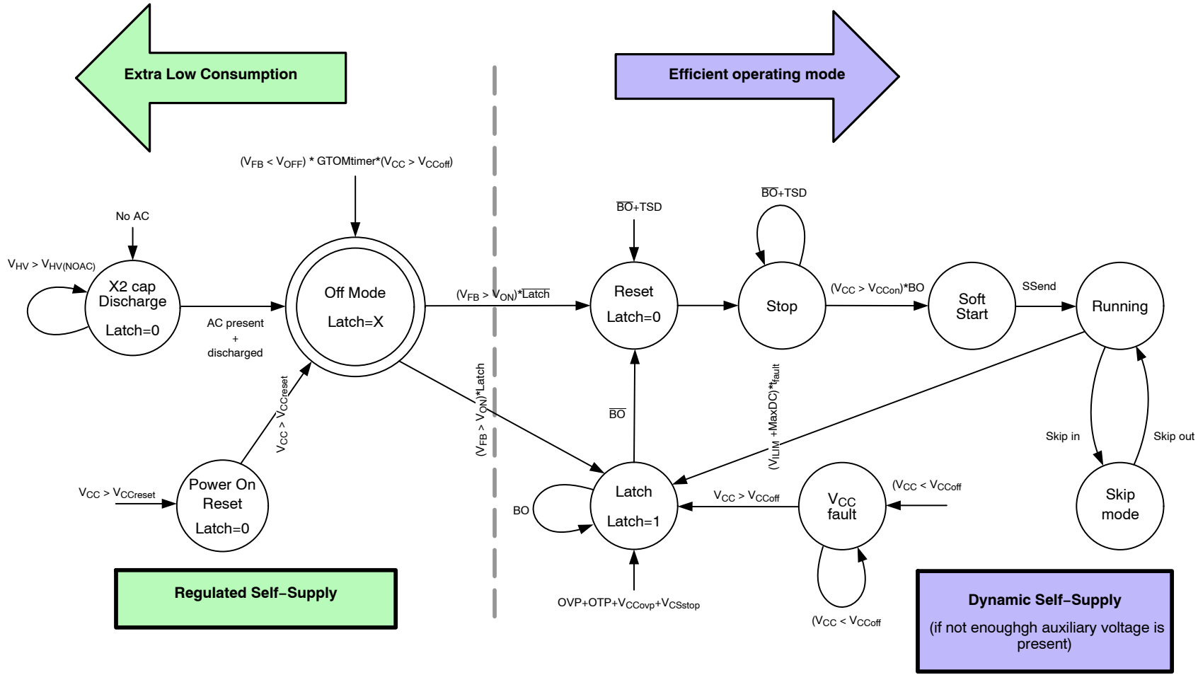
Figure 46. Operating Status Diagram for the Fully Latched Versions A/C of the Device
