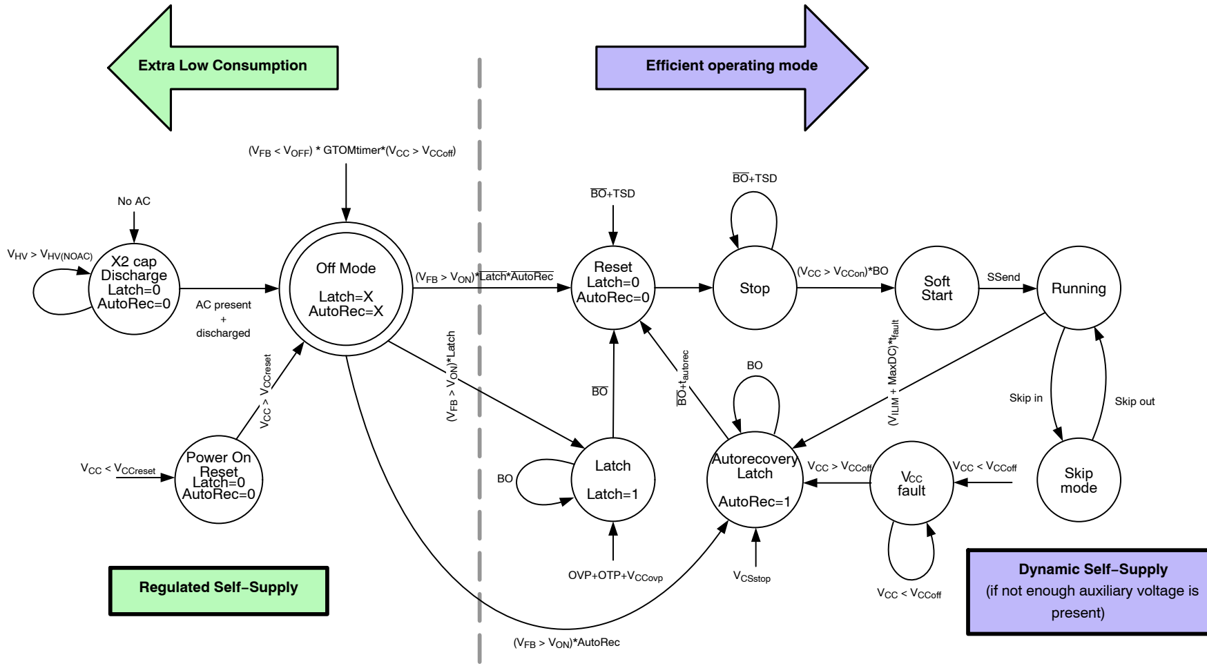
Figure 47. Operating Status Diagram for the Autorecovery Versions B/D of the Device
