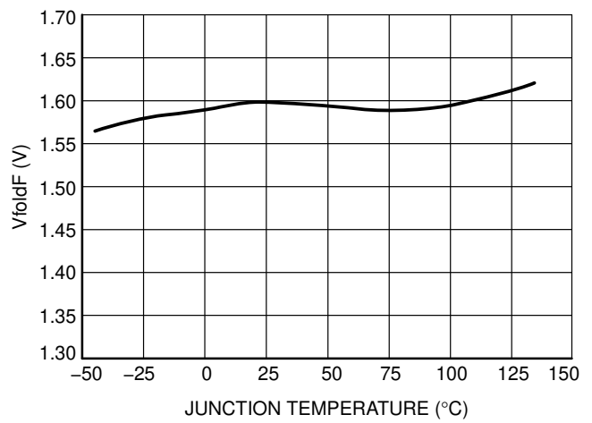
Figure 22. VfoldF vs. Junction Temperature
