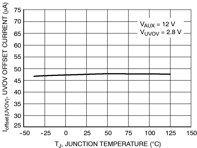
Figure 11. UV/VOV Offset Current vs. Junction Temperature
