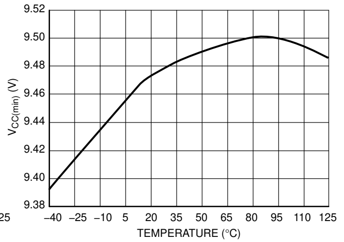
Figure 5. V_{CC(min)} Threshold
