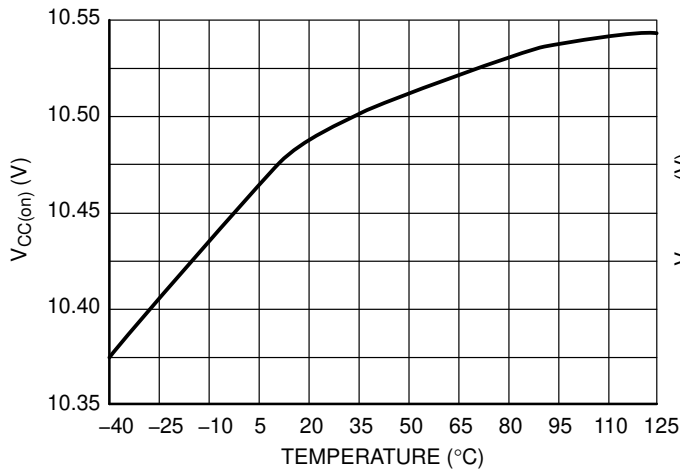
Figure 4. V_{CC(on)} Threshold
