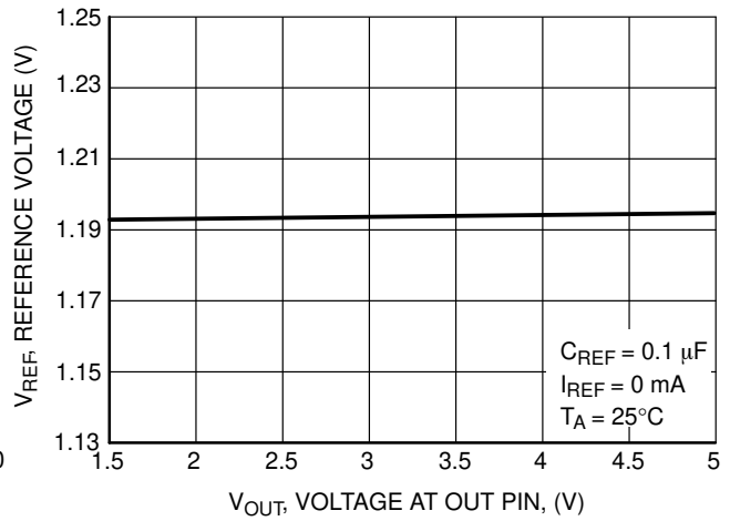
Figure 4. Reference Voltage vs. Voltage at OUT Pin
