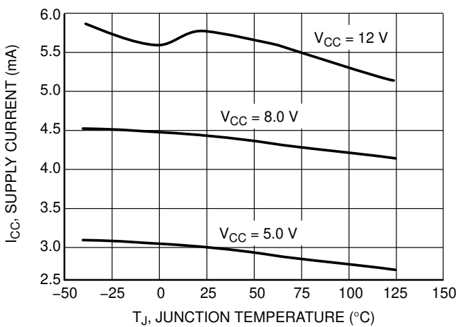
Figure 8. Quiescent Current ( I_{CC} ) vs. Temperature (Switching)
