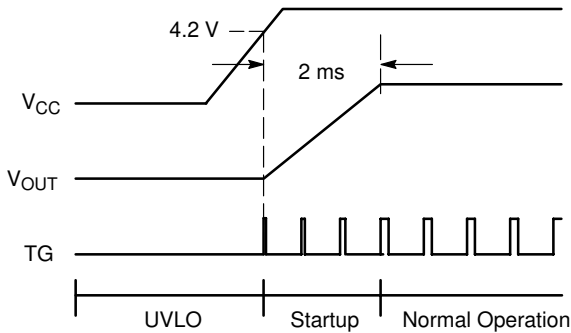
Figure 10. Normal Startup
