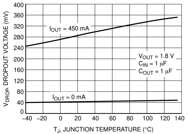
Figure 20. Dropout Voltage vs. Temperature – V_{OUT} = 1.8 V
