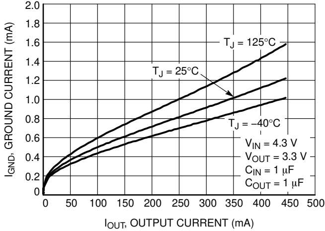
Figure 15. Ground Current vs. Load Current – V_{OUT} = 3.3 V
