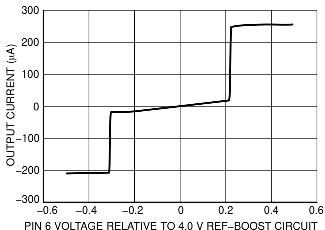
Figure 10. Voltage Amplifier Gain
