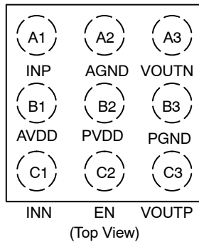
Figure 1. Pin Description
