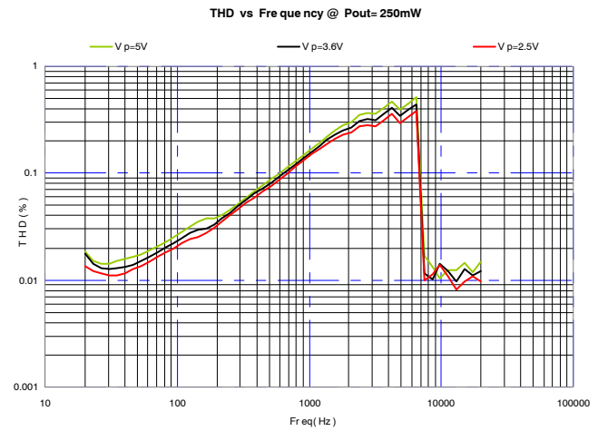
Figure 7. THD vs. Frequency, R_I = 8 \Omega , P_{OUT} = 250 \text{ mW}
