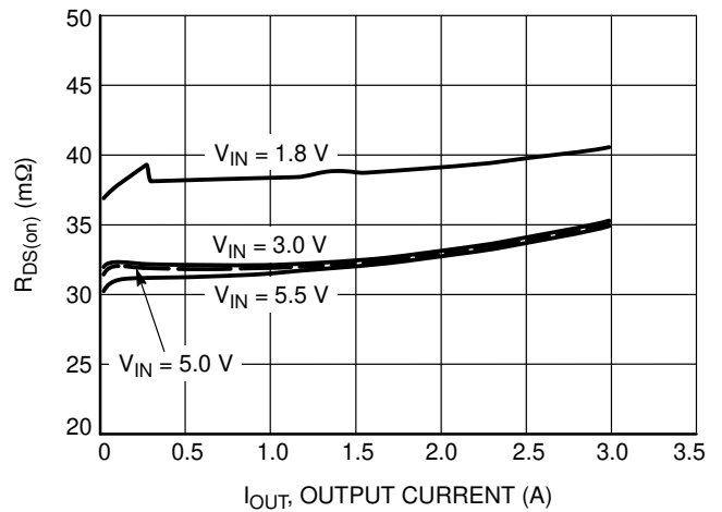
Figure 8. R_{DS(on)} vs. I_{OUT} at 25^\circ C
