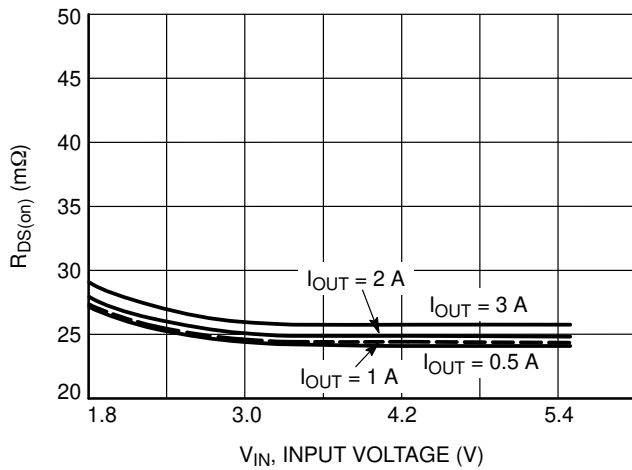
Figure 7. R_{DS(on)} vs. V_{IN} Voltage at -40^\circ C
