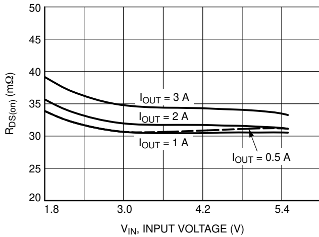
Figure 5. R_{DS(on)} vs. V_{IN} Voltage at 25^\circ C
