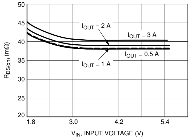
Figure 6. R_{DS(on)} vs. V_{IN} Voltage at 85^\circ C
