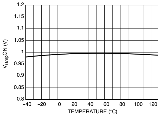
Figure 10. V rampON versus Temperature @ V pin5 = 2.0 V
