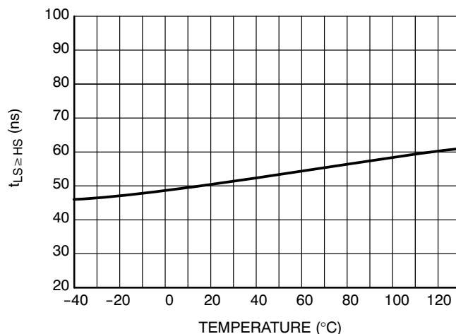
Figure 12. Low-Side to High-Side Delay versus Temperature, High-Side Rising
