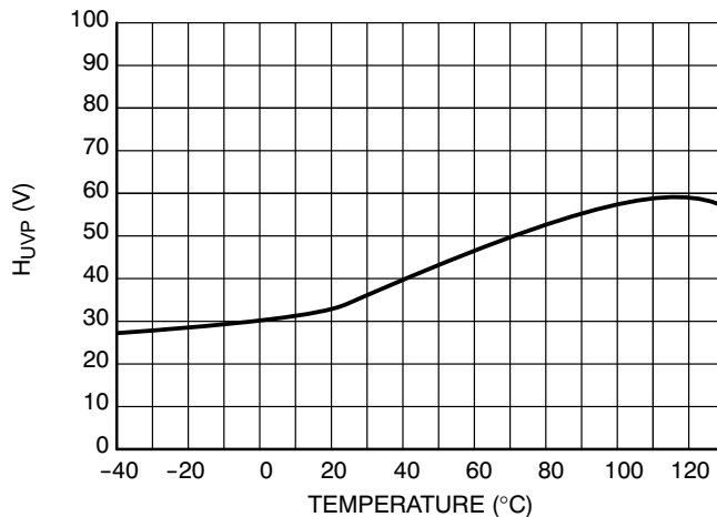
Figure 14. Hysteresis of the UVP Comparator versus Temperature
